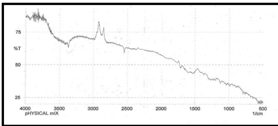
Fig no 4: Overlapping IR Spectra of physical mixture and API.
