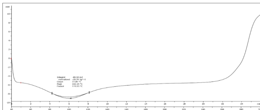
Fig No 6: DSC thermogram of Na-CMC
