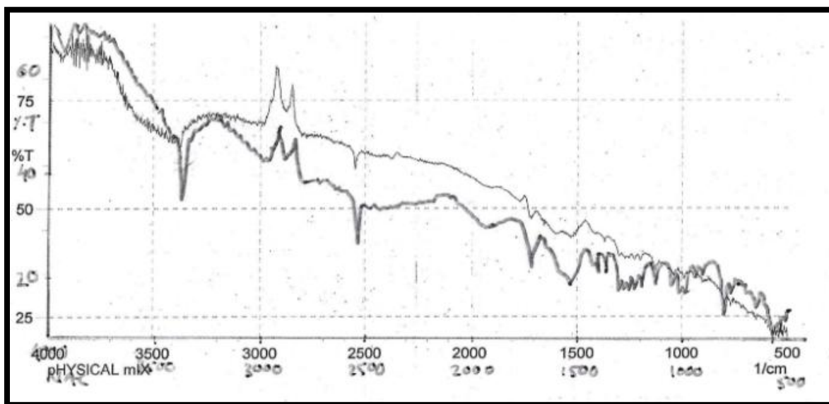
Fig no 4: Overlapping IR Spectra of physical mixture and API.
