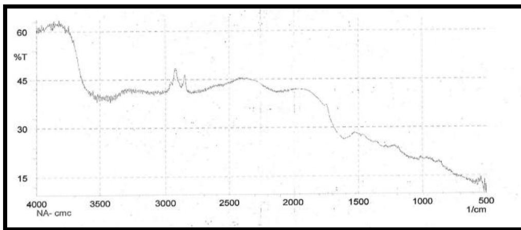
Fig no 3: IR Spectra of Physical mixture.
