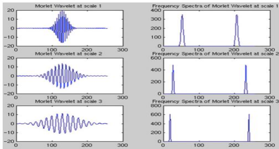
Fig.11: The Morlet Wavelet [24]
