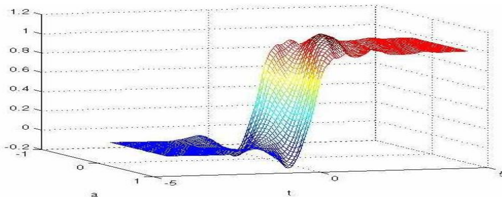
Fig. 6: Gibbs function of Daubechies Wavelet where N=4[22].
