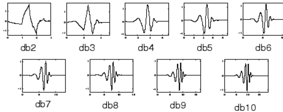
Fig. 5: Daubechies Wavelets db2 on the Left and db10 on the Right [6].
