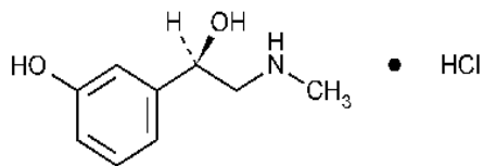
Fig. 3: Phenylephrine HCL (PEH)
