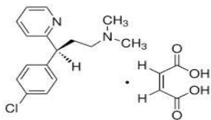
Fig. 1: Chlorpheniramine Maleate (CPM)
