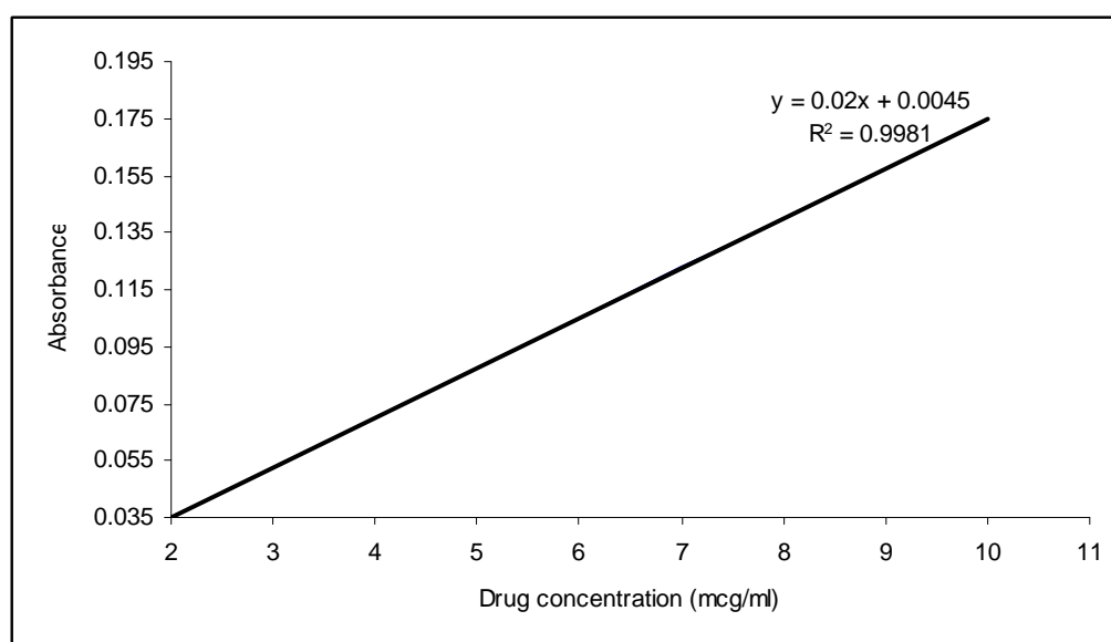
Fig. 2: Calibration curve of Lamivudine by the proposed method
