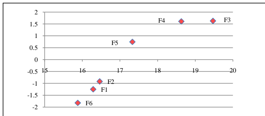
Figure 6. Cause and Effect Relationship among the Six Factors.
