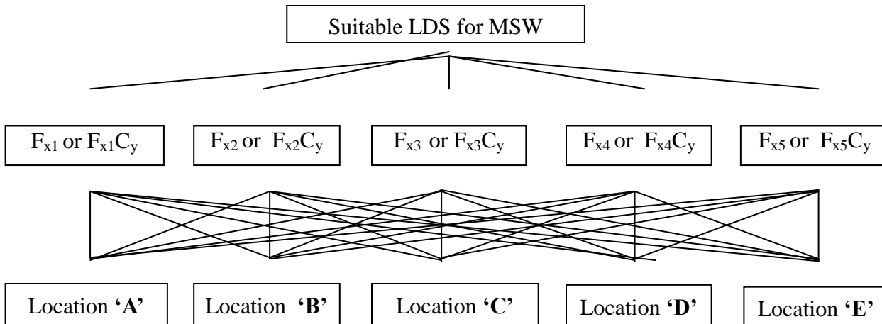
Figure 4: The Proposed Hierarchy Structure of “AHP”.
