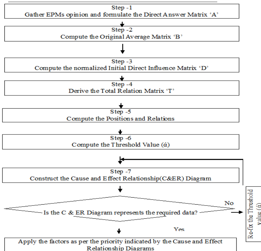
Figure 2 DEMATEL Application Procedure.
