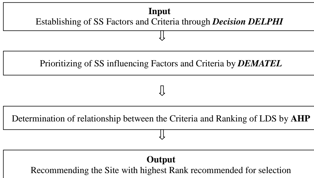
Figure 1. Research Design of Hybrid DEMATEL and AHP
