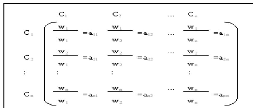
Figure 5. Comparison Reciprocal Matrix.
