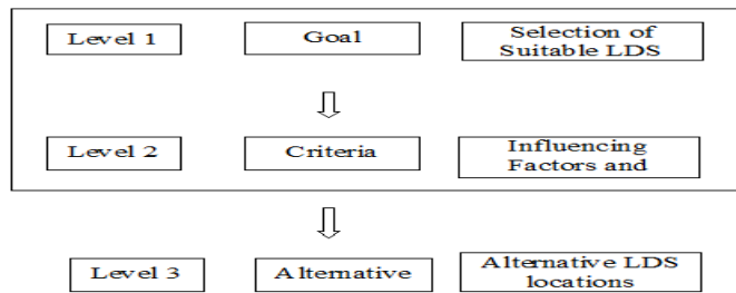
Figure 3, Model Linear Hierarchy of “AHP”
