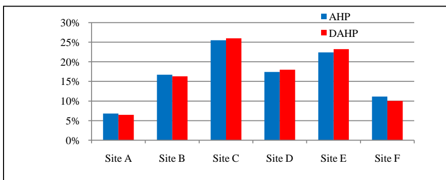
Figure 7 Final Ranking of LDS.
