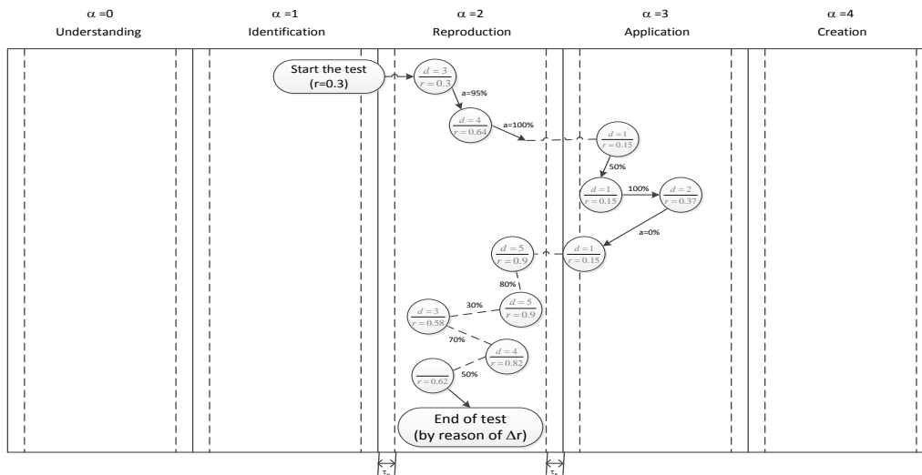
Fig. 4. Example of algorithm to generate questions in the adaptive learning system.
