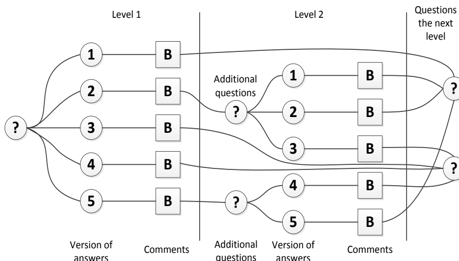
Fig. 2. The structure of the test in the algorithmic approach.
