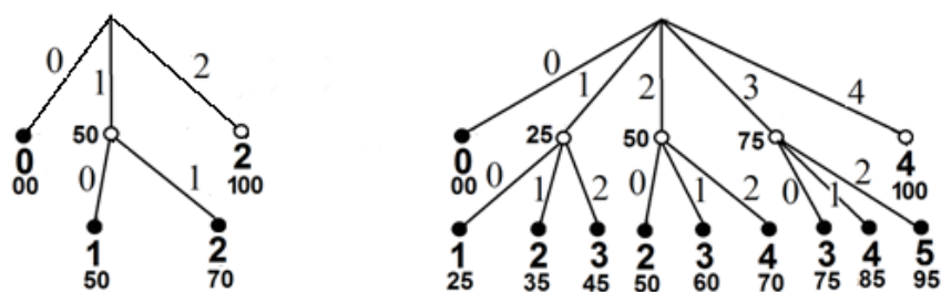
Fig. 3. Driving a single-stage testing algorithm.
