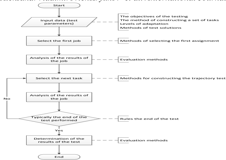
Fig. 1. The template algorithm of the adaptive testing system.
